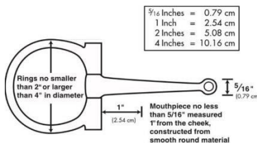
SNAFFLE BIT WITH CONNECTING FLAT BAR
